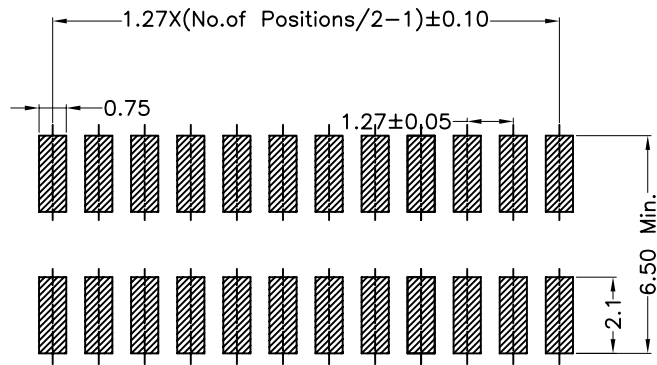
PCB Layout
