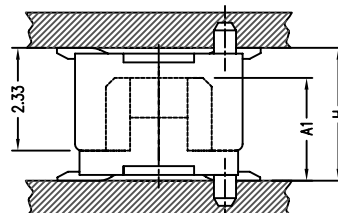
Mating Drawing (Ref)
