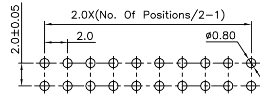
PCB Layout
