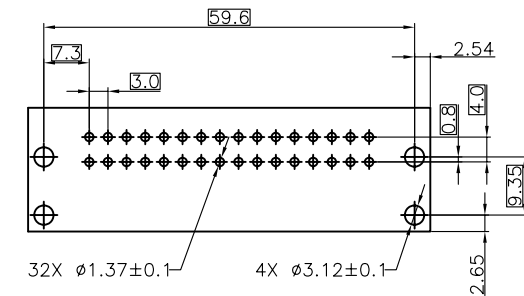
MATING CIRCUIT BOARD DETAIL CONNECTOR MATING SIDE
