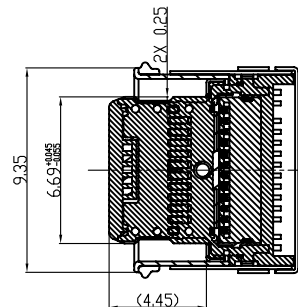
SECTION H-H SCALE (1:1)
