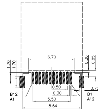
RECOMMENDED P.C.B. LAYOUT (T:1.00mm) TOLERANCE UNSPECIFIED ±0.05mm
