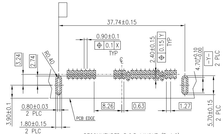
RECOMMENDED P.C.B LAYOUT (T=1.2)
