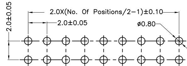
PCB Layout
