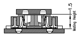
MATED DRAWING (REF) SCALE : 5 : 1
