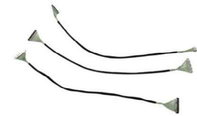
HRS:DF80-50P-0.5SD(51)*2 Wire Harness
